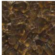
Copper crystals
